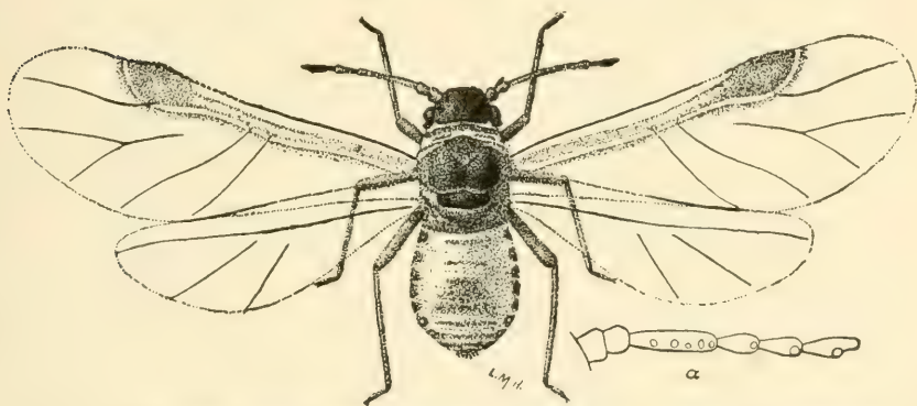
FIG. 122.—Grass root-lice ( Schizoneura panicola ); winged viviparous female. a , antenna. (After Forbes.)
